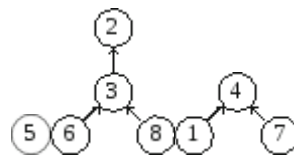
Fig. 7.41 A union-find structure with three sets
