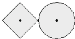
Fig. 13.13 Two distance functions
