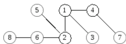
FIG. 10.1 A tree that consists of 8 nodes and 7 edges
