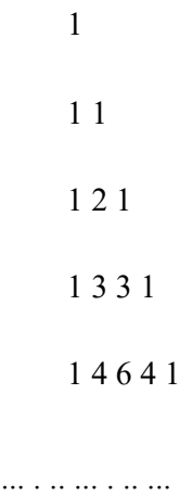
Fig. 11.4 First 5 rows of Pascal’s triangle
