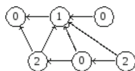
Fig. 11.23 Grundy numbers of game states
