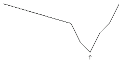
FIG. 8.7 A function and its minimum value
