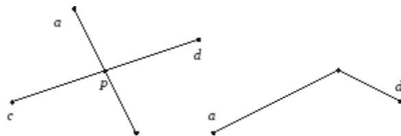
FIG. 13.6 Case 3: the line segments have an
