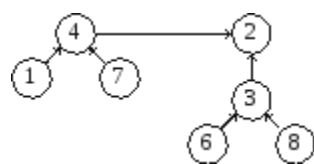
Fig. 7.42 Joining two sets into a single set
