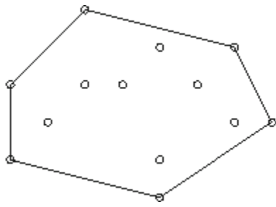
Fig. 13.22 Convex hull of a point set
