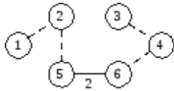
Fig. 7.40 Including the edge 5–6 reduces the weight of the spanning tree
