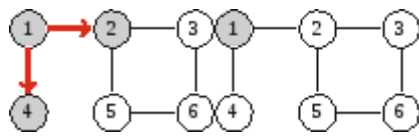
Fig. 7.14 Breadth-first search
