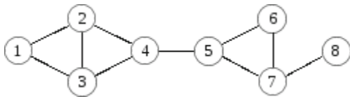
FIG. 12.41 A graph with three articulation points and two bridges
