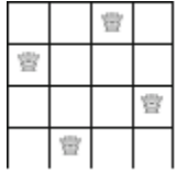
Fig. 2.2 The possible ways to place 4 queens on a 4 \times 4 chessboard
