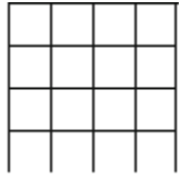
Fig. 3.4 Possible positions for queens on the last row and column
