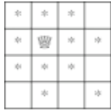
Fig. 3.3 The queen attacks all squares marked with “*” on the board
