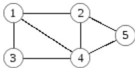
FIG. 7.1 A graph with 5 nodes and 7 edges
