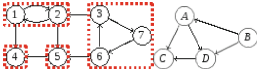
FIG. 12.2 A graph, its strongly connected components and the component graph
