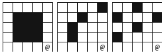
Fig. 11.26 A game that consists of three subgames
