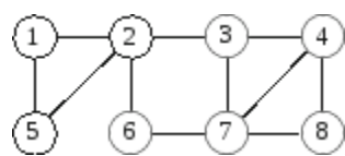
Fig. 12.43 A graph and an Eulerian subgraph
