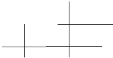
FIG. 13.17 Five line segments with three intersection points
