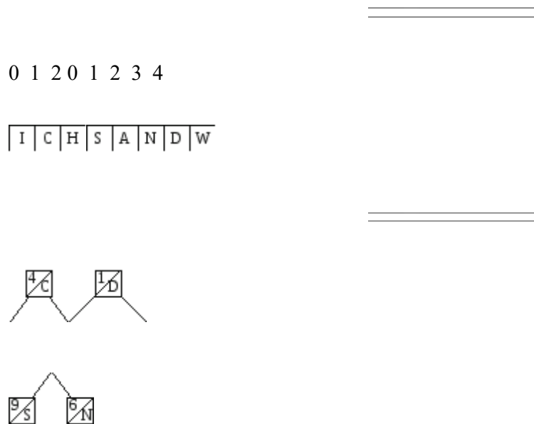
FIG. 15.21 Merging two arrays into an array, after merging
