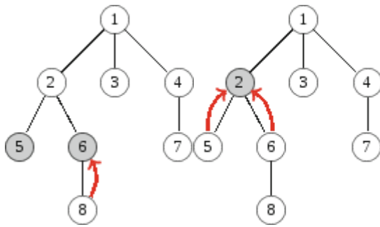
Fig. 10.20 Two steps to find the lowest common ancestor of nodes 5 and 8
