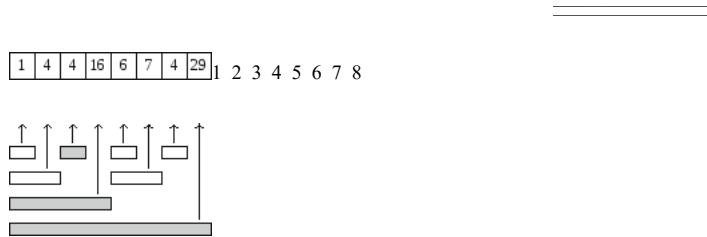
Fig. 9.9 Updating a value in a binary indexed tree
