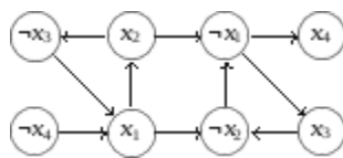
Fig. 12.6 The implication graph of L_1
