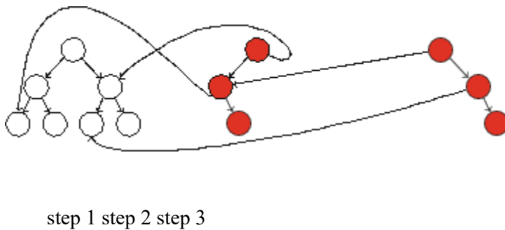
Fig. 15.15 A compact way to store the modification history
