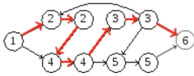
Fig. 12.26 A construction that limits the flow through the nodes
