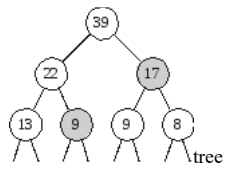
Fig. 9.11 Processing a range sum query using a segment
