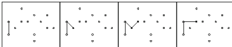
Fig. 13.22 Convex hull of a point set
