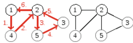
Fig. 12.10 A graph and an Eulerian circuit
