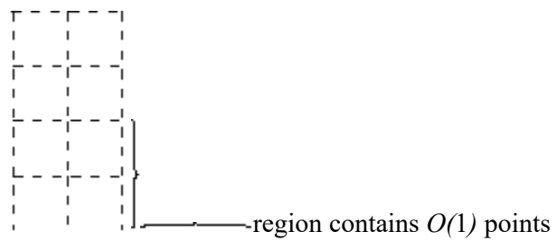
Fig. 13.21 Closest point d
