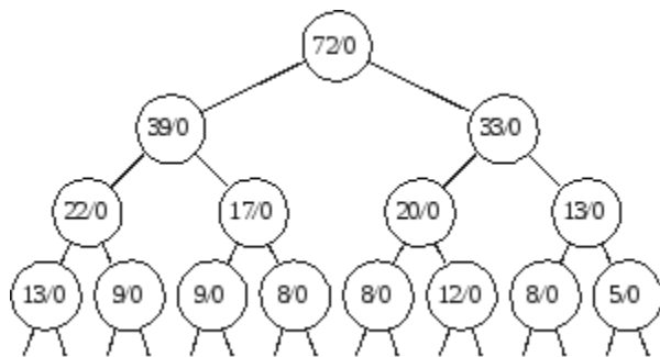
Fig. 15.9 Traversing a segment tree from top to bottom
