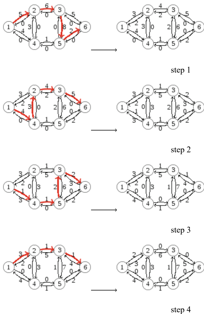
Fig. 12.21 The Ford–Fulkerson algorithm
