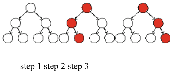
Fig. 15.14 A modification history of a segment tree: the initial tree and two updates
