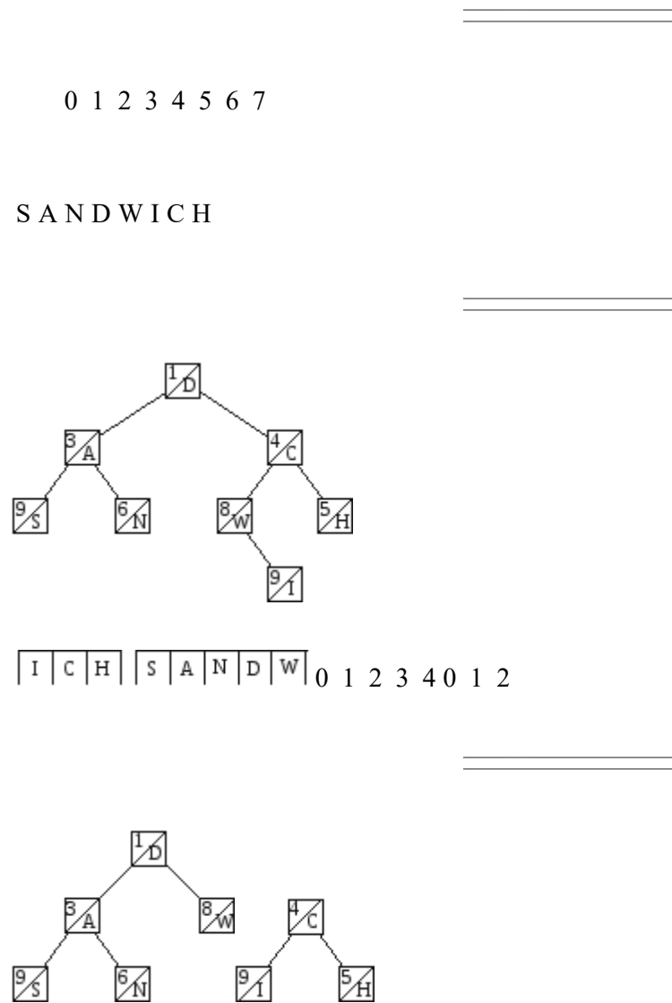
Fig. 15.19 Splitting an array into two arrays
