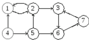
FIG. 12.3 The processing order of the nodes
