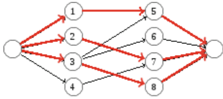
Fig. 12.28 Maximum matching as a maximum flow
