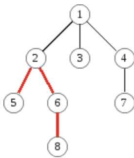
Fig. 10.22 Finding the lowest common ancestor of nodes 5 and 8
