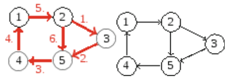
Fig. 12.11 A directed graph and an Eulerian path
