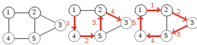
Fig. 12.13 A graph, a Hamiltonian path and a Hamiltonian circuit
