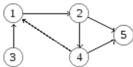
FIG. 7.7 A directed graph
