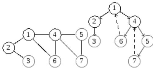
Fig. 12.39 A graph and its depth-first search tree
