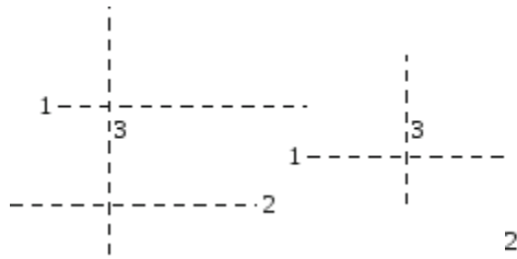
Fig. 13.18 Events that correspond to the line segments
