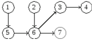
Fig. 12.33 An example graph for constructing path covers
