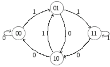
Fig. 12.14 Constructing a De Bruijn sequence from an Eulerian path
