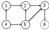
Fig. 7.24 A graph and a topological sort
