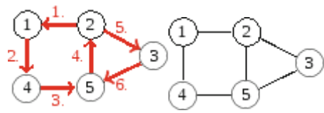
Fig. 12.9 A graph and an Eulerian path
